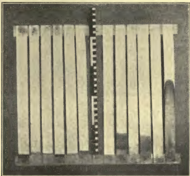
FIG. 7.—Ascent of positively and negatively charged colloids. (According to N. Sahlbom.)
